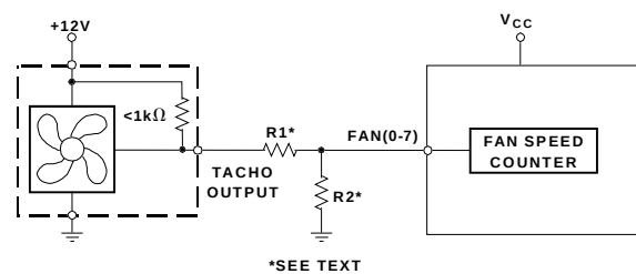
Figure 13d. Fan with Strong Tach. Pullup to >V_{CC} or Totem-Pole Output, Attenuated with R1/R2
