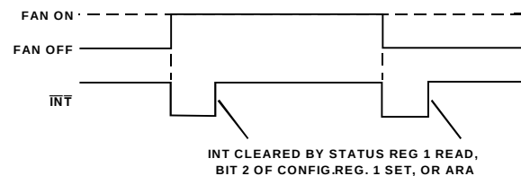
Figure 19. Assertion Of INT Due To AFC Event
