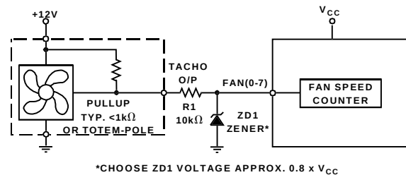
Figure 13c. Fan with Strong Tach. Pullup to >V_{CC} or Totem-Pole Output, Clamped with Zener and Resistor
