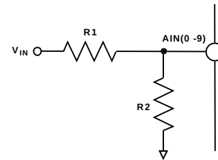
Figure 6. Scaling AIN(0 - 9)
