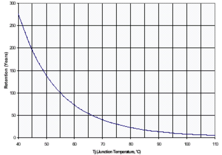
Figure 2. E 2 PROM Memory Retention
