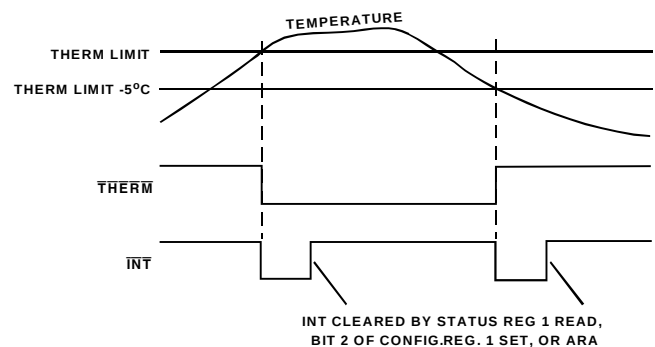
Figure 20. Assertion Of \overline{\text{INT}} Due To \overline{\text{THERM}} Event
