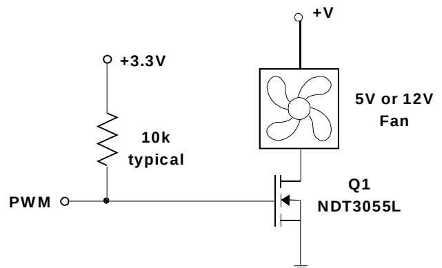
Figure 11f. PWM Fan Drive Circuit using an N-Channel MOSFET
