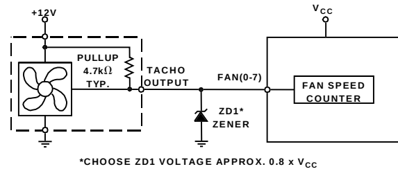
Figure 13b. Fan with Tach. Pullup to Voltage >V_{CC} e.g. 12\text{V} Clamped with Zener Diode
