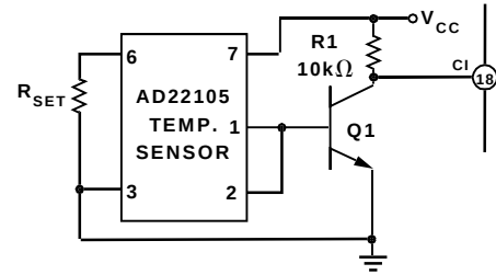
Figure 15. Using the CI Input with a Temperature Sensor
