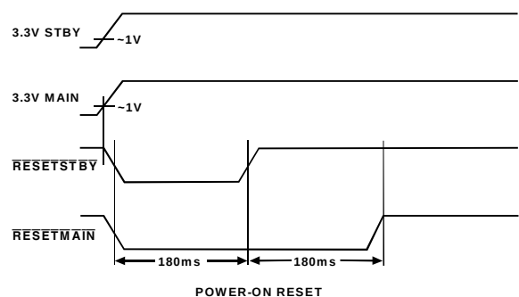
Figure 21. Operation Of Reset Outputs
