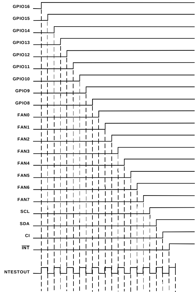
Figure 23. NAND Tree Test Taking Inputs High In Turn
