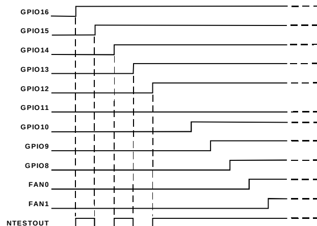
Figure 25. NAND Tree Test With GPIO11 Stuck Low
