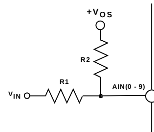
Figure 7. Scaling and Offsetting AIN(0 - 9) for Negative Inputs
