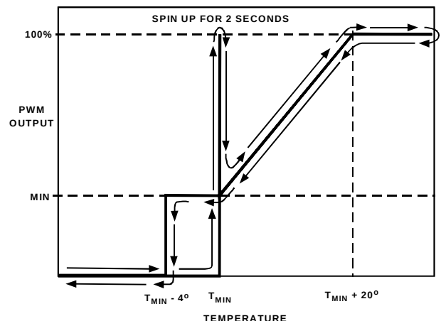
Figure 12a. Automatic PWM Fan Control Transfer Function
