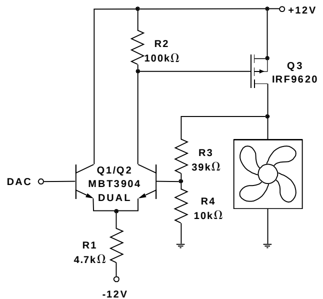
Figure 11e. Discrete Fan Drive Circuit with P-Channel MOSFET, Dual Supply
