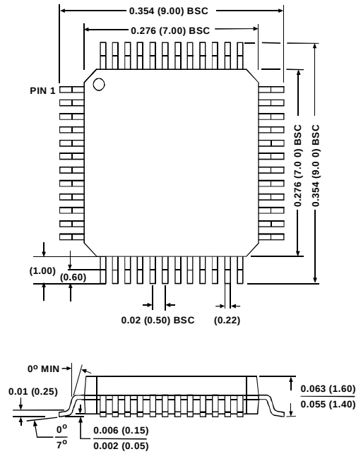
48-Pin LQFP Package (ST-48)
