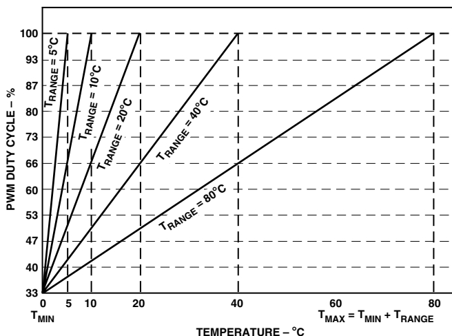
Figure 7. PWM Duty Cycle vs. Temperature Slopes ( T_{RANGE} )
