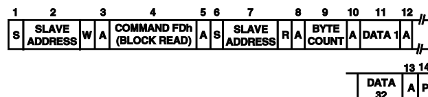
Figure 47. Block Read From EEPROM or RAM
