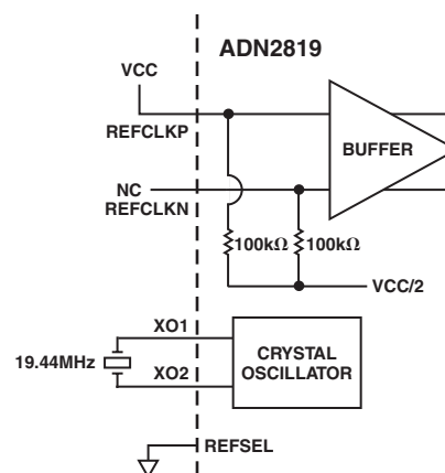
Figure 17. Crystal Oscillator Configuration
