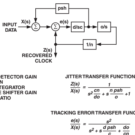
Figure 13. PLL/DLL Architecture
