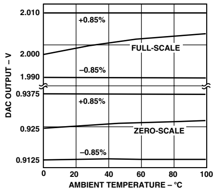
TPC 4. DAC Output Voltage vs. Temperature
