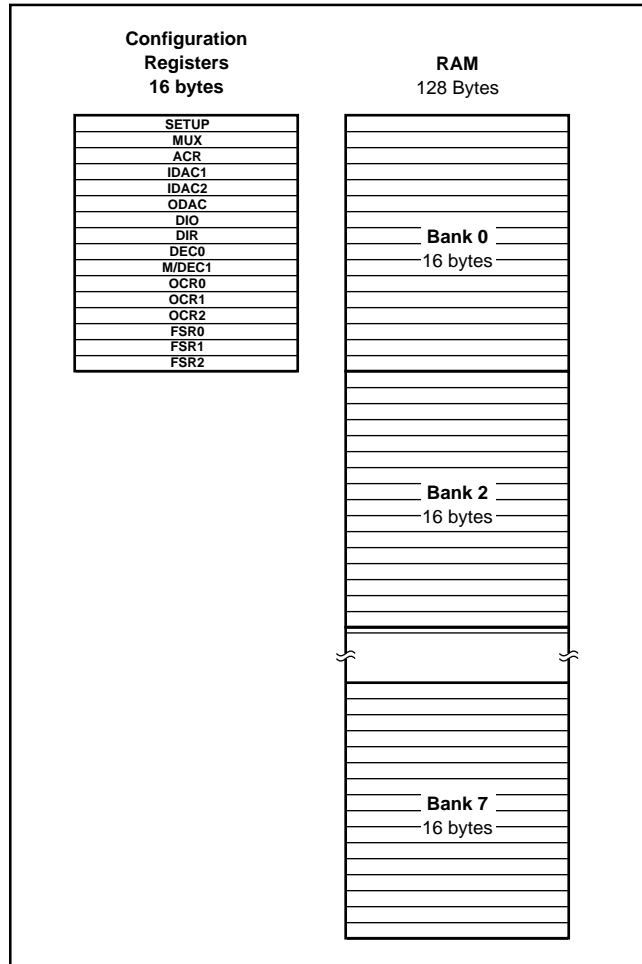
FIGURE 5. Memory Organization.
