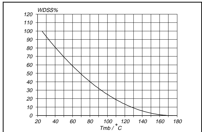
Fig.15. Normalised avalanche energy rating. W_{DSS}\% = f(T_{mb}) ; conditions: I_D = 9 \text{ A}
