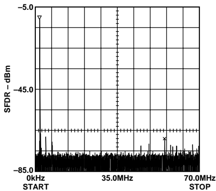
Figure 17. Single-Tone SFDR @ f_{CLOCK} = 140\text{ MHz} ( f_{OUT1} = 2\text{ MHz} )
