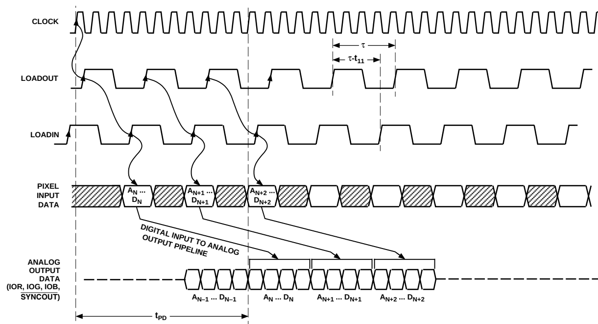
Figure 8. Pixel Input to Analog Output Pipeline with Maximum \text{LOADOUT} to \text{LOADIN} Delay (4:1 Multiplex Mode)
