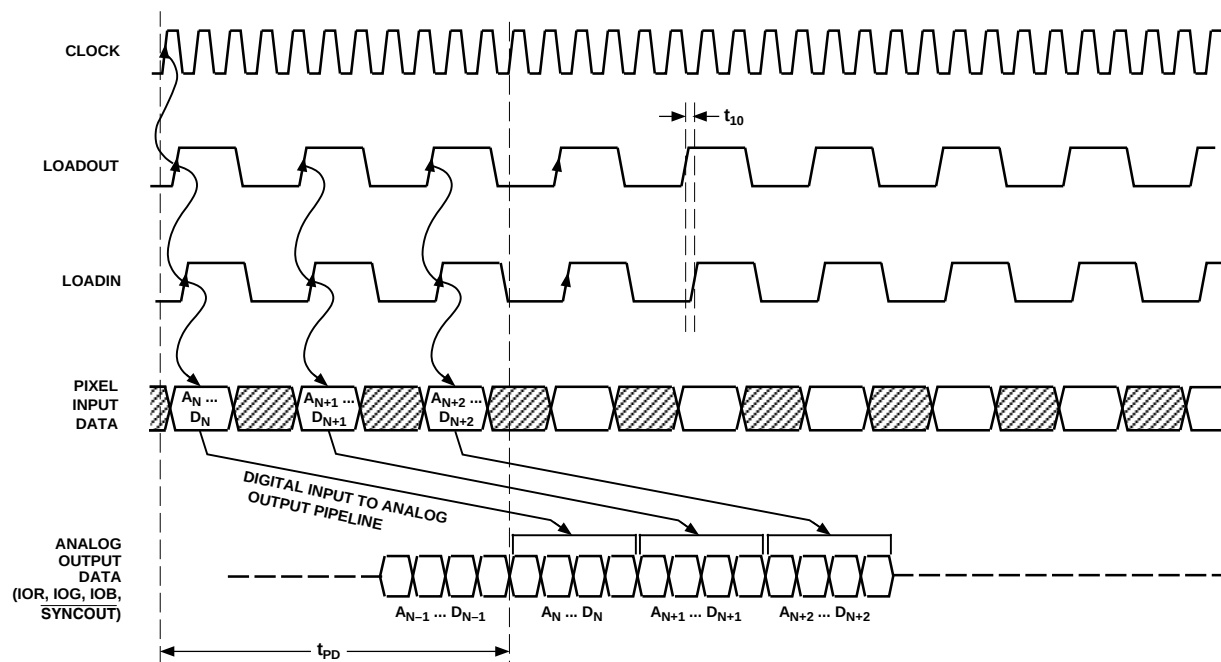
Figure 7. Pixel Input to Analog Output Pipeline with Minimum \text{LOADOUT} to \text{LOADIN} Delay (4:1 Multiplex Mode)
