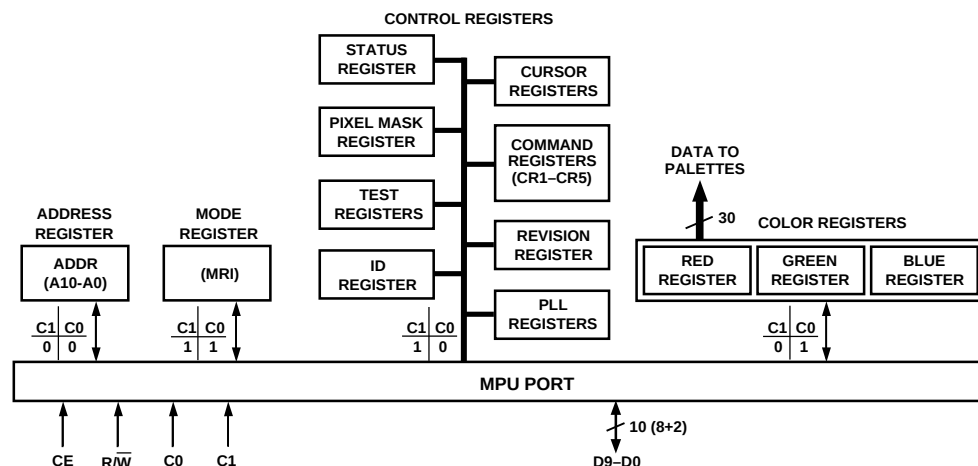
Figure 33. MPU Port and Register Configuration
