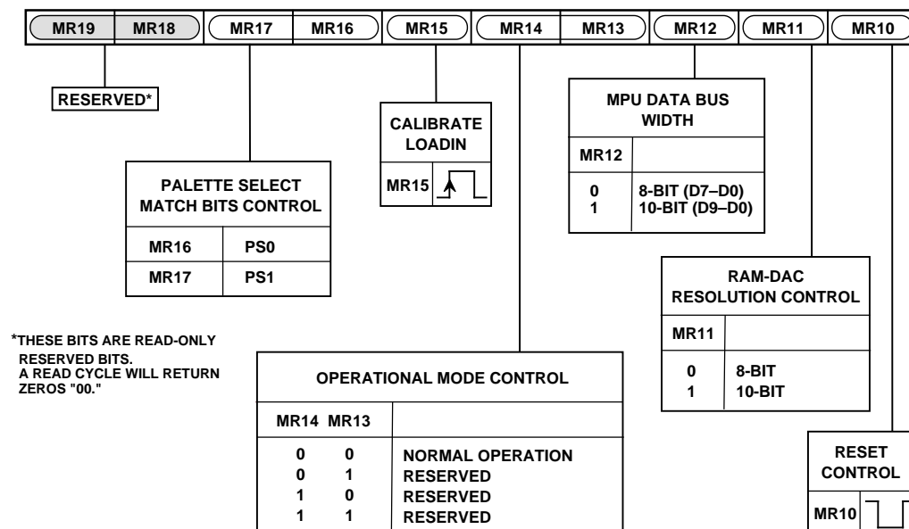
Figure 39. Mode Register 1 (MR1) (MR19–MR10)
