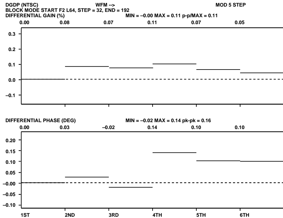
Figure 82. NTSC Differential Gain and Phase Measurement
