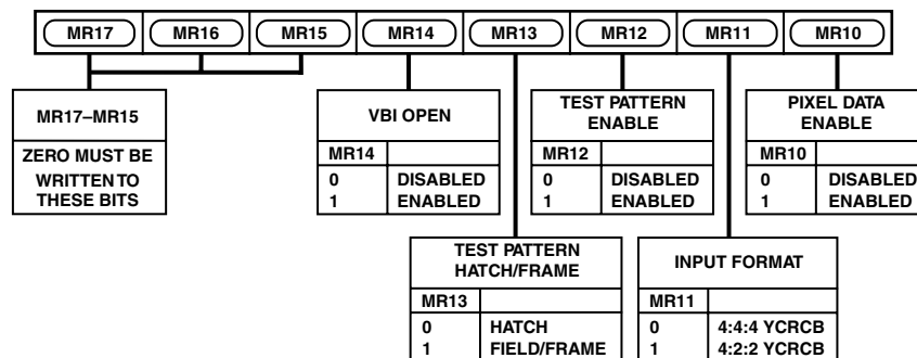
Figure 51. Mode Register 1
