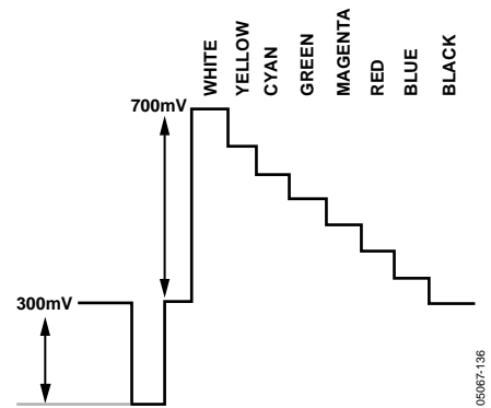
Figure 134. Y Levels—NTSC
