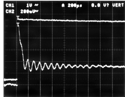
Figure 11. Typical Self-Test Response at V_{DD} = 5\text{ V}
