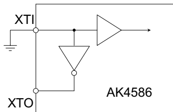
Figure 5. Off mode
