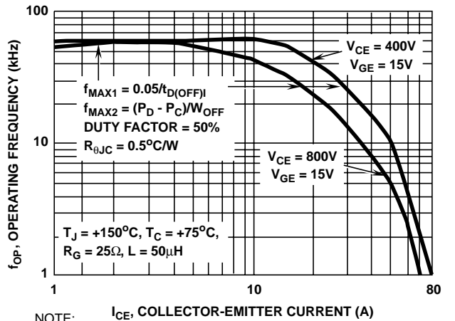
FIGURE 10. OPERATING FREQUENCY vs COLLECTOR-EMITTER CURRENT AND VOLTAGE
