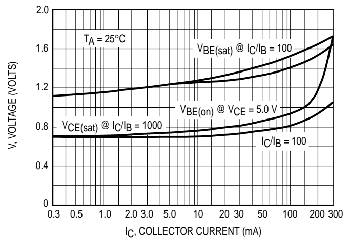
Figure 3. "On" Voltage
