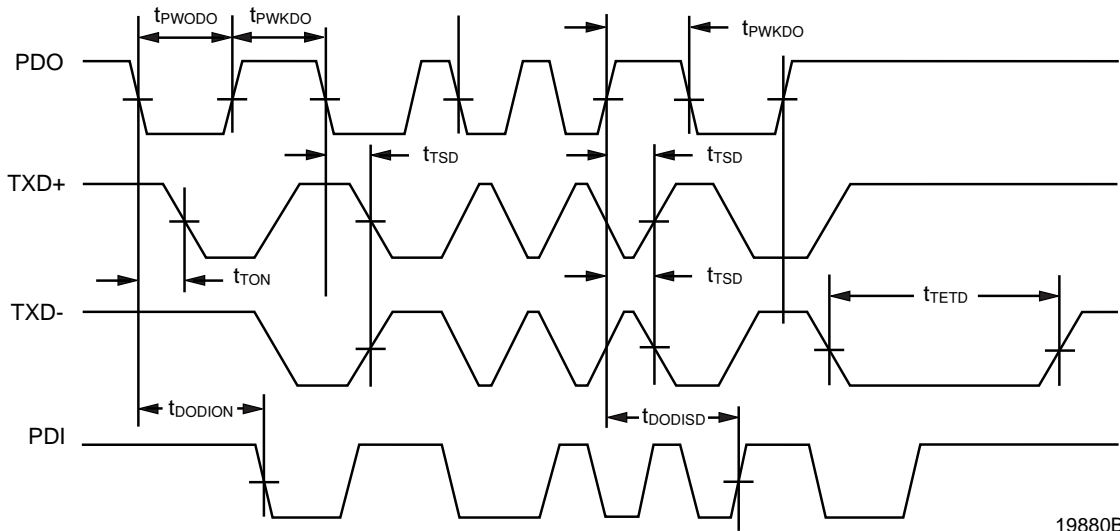
Figure 9. Transmit Signals
