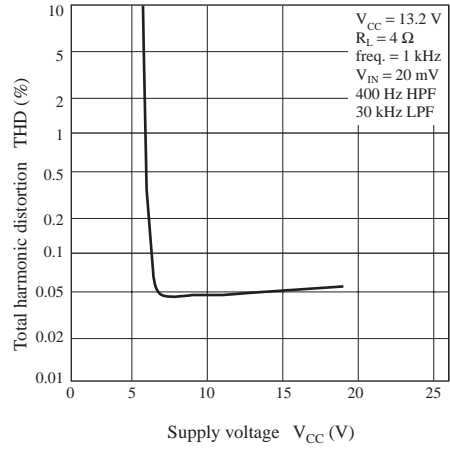
THD — V_{CC}
