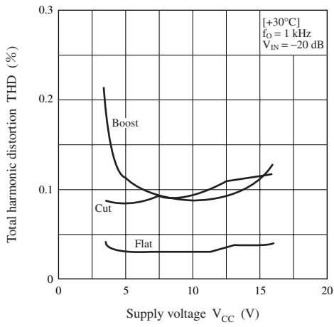
THD — V_{CC}
