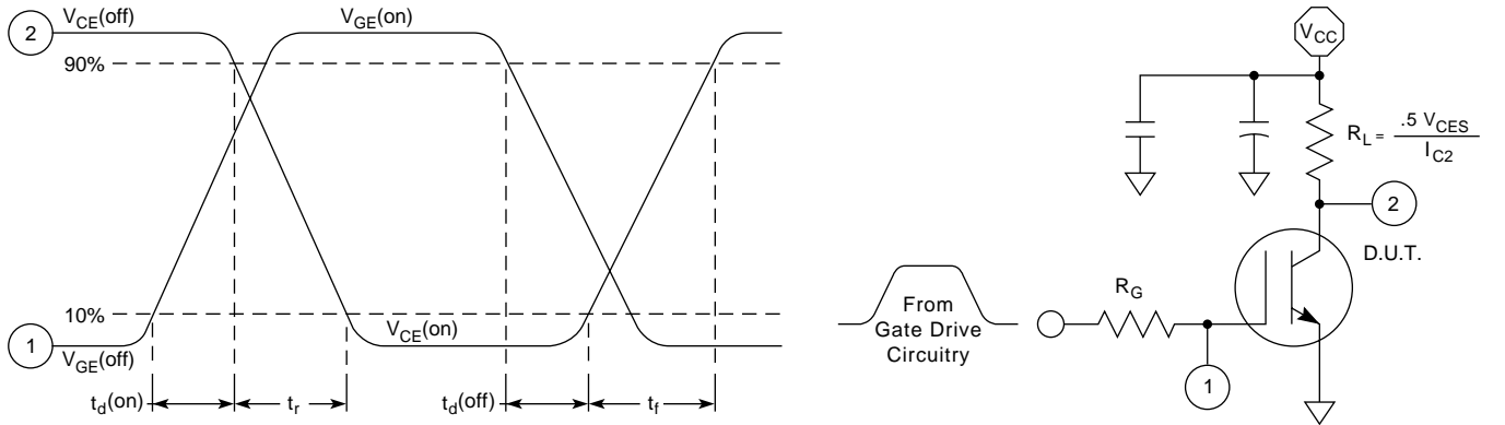
Figure 16, Resistive Switching Time Test Circuit and Waveforms
