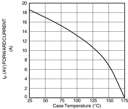
Figure 28. Current Derating
