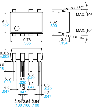
Through hole terminal type
