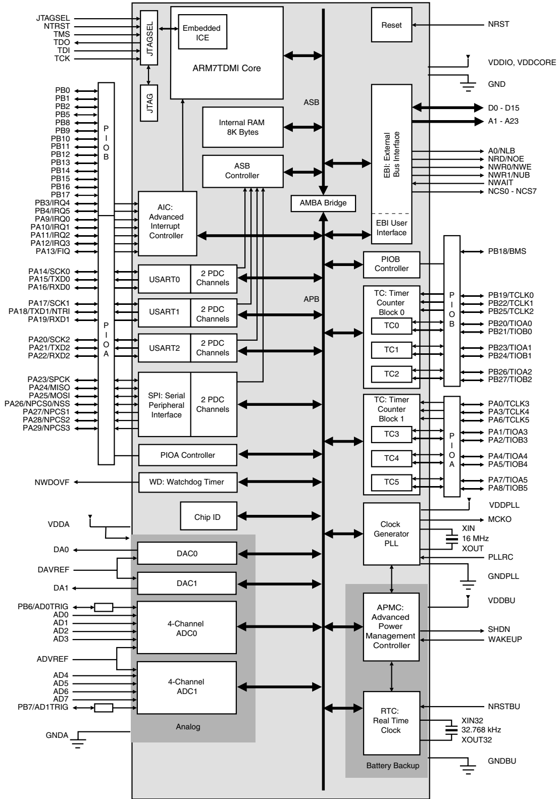
Figure 3. AT91M55800A
