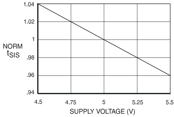
NORMALIZED t_{SIS} vs. SUPPLY VOLTAGE (TA = 25°C)
