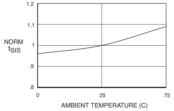
NORMALIZED t_{SIS} vs. AMBIENT TEMPERATURE (V CC = 5V)
