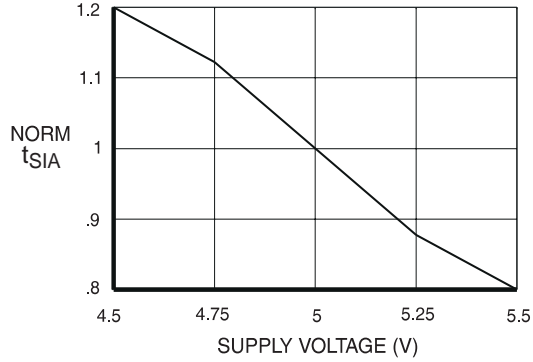
NORMALIZED t_{SIA} vs. SUPPLY VOLTAGE (TA = 25°C)
