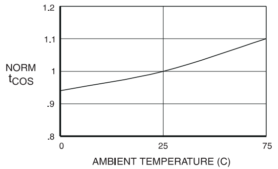
NORMALIZED t_{COS} vs. AMBIENT TEMPERATURE ( V_{CC} = 5V )
