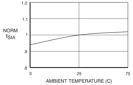
NORMALIZED t_{SIA} vs. AMBIENT TEMPERATURE (V CC = 5V)
