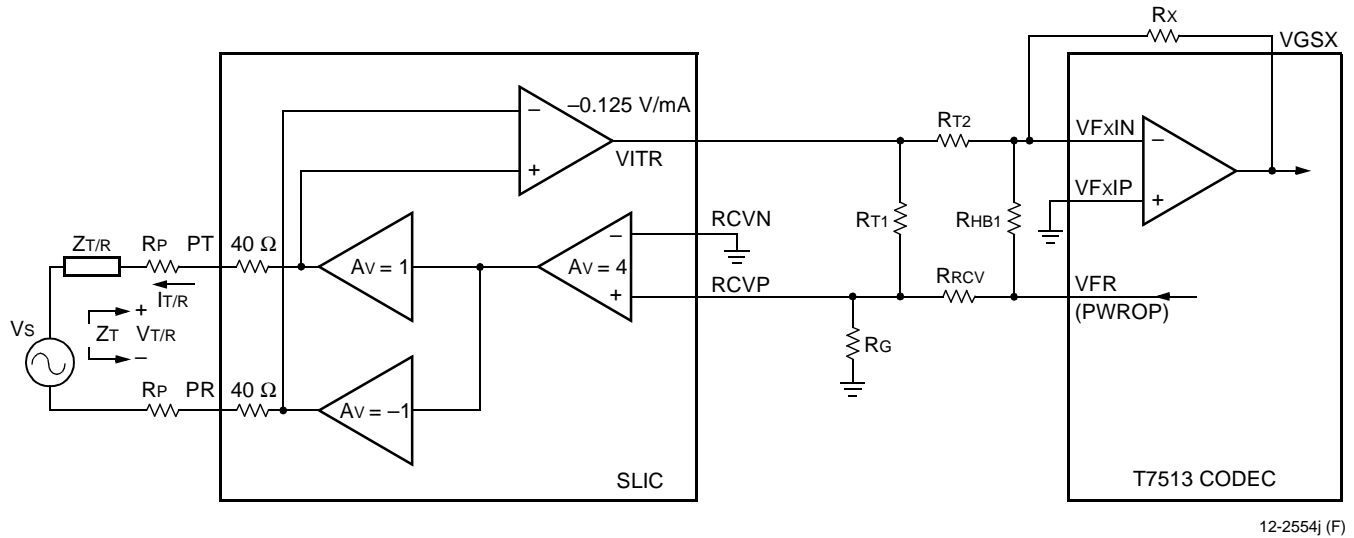
Figure 32. ac Equivalent Circuit Not Including Spare Op Amp
