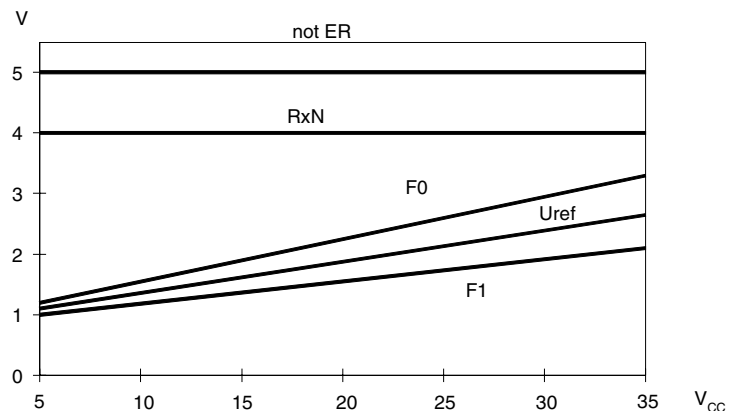
Figure 7. Comparator Thresholds
