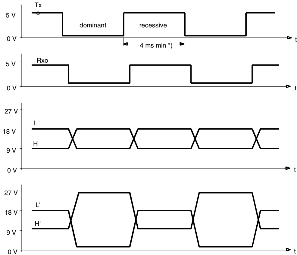
Figure 3. Pulse Diagram
