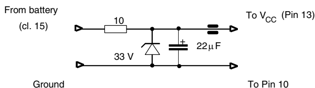
Figure 6. Implementation of a Power Filter and Over Clamps
