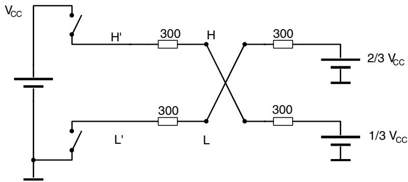
Ideal test circuit equivalent
