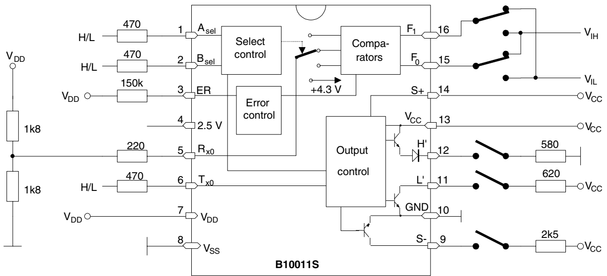
Figure 4. Test Circuit
