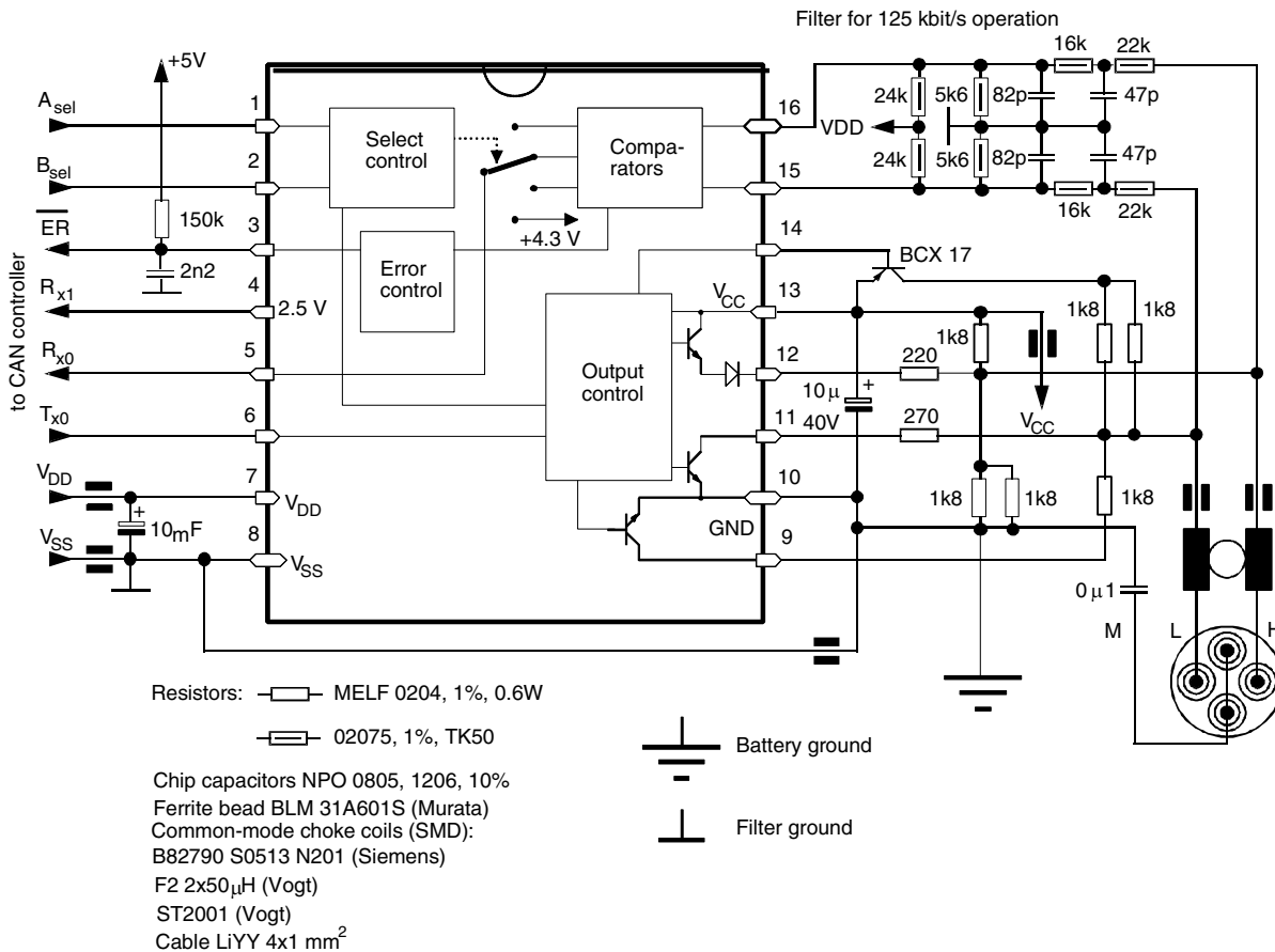
Figure 5. Application Circuit
