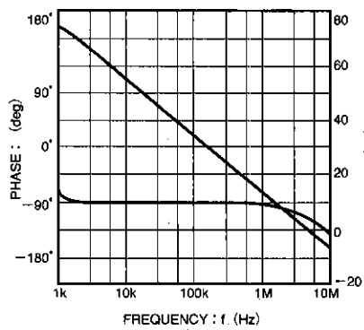
Fig. 9 Operational amplifier vs. open loop characteristics
