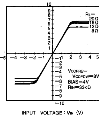
Fig. 11 Driver I/O characteristics (variable load)
