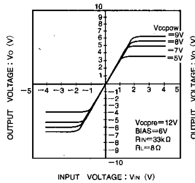
Fig. 10 Driver I/O characteristics (variable V_{CCPOW} )
