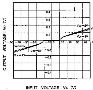
Fig. 7 Dead zone I/O characteristics
