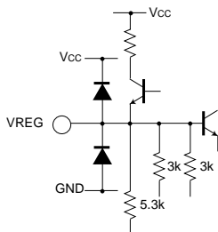
31pin (36pin)
