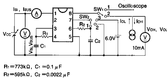
Fig. 5 Measurement circuit (1)
