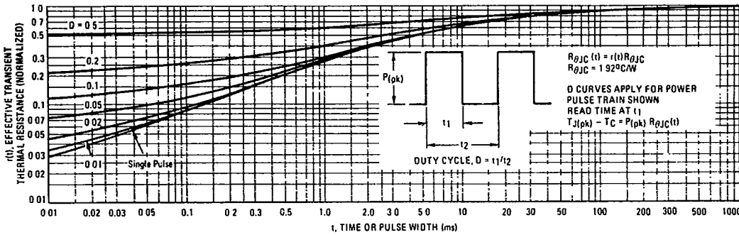
FIGURE 4 - THERMAL RESPONSE
