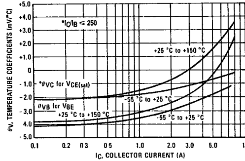
FIGURE 12 - TEMPERATURE COEFFICIENTS
