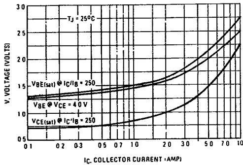
FIGURE 11 - "ON" VOLTAGES
