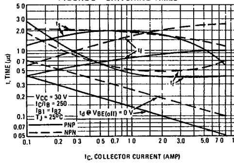
FIGURE 3 - SWITCHING TIMES
