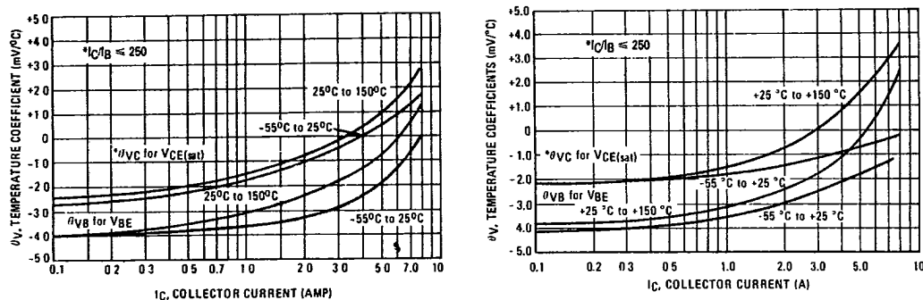
FIGURE 12 — TEMPERATURE COEFFICIENTS
