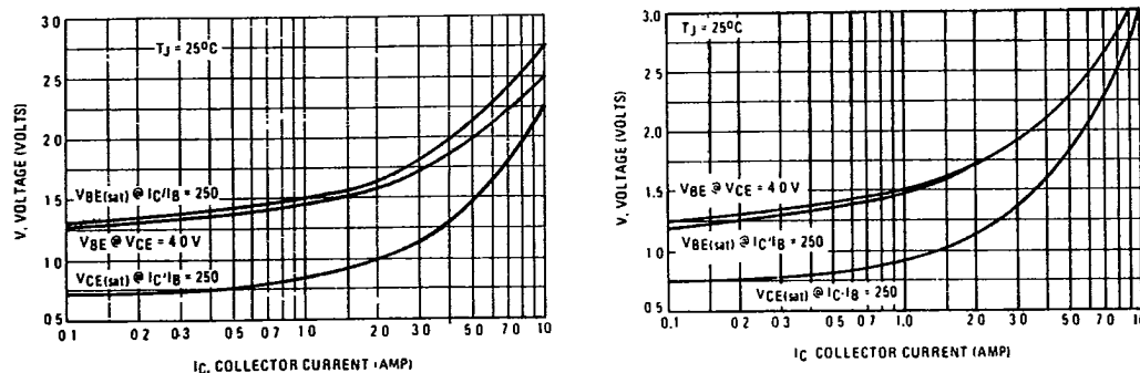
FIGURE 11 — "ON" VOLTAGES
