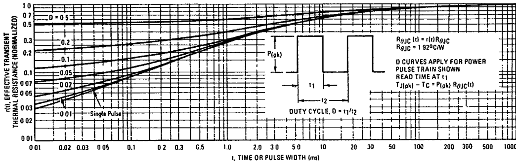
FIGURE 4 - THERMAL RESPONSE
