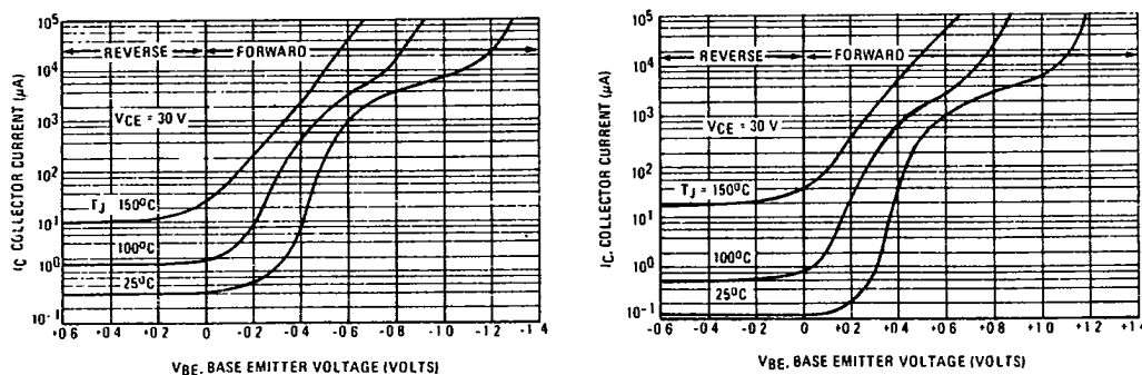
FIGURE 13 — COLLECTOR CUT-OFF REGION
