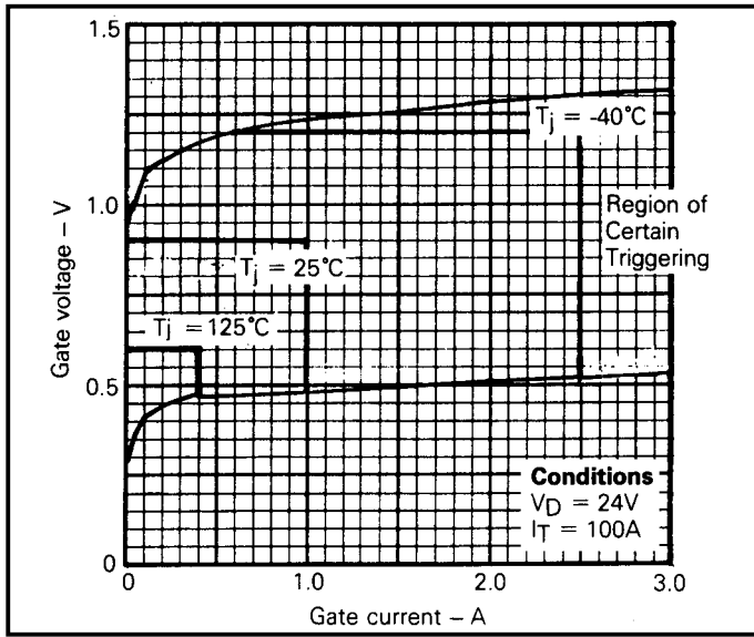
Fig.1 Gate characteristics
