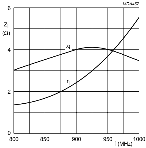
Fig.10 Input impedance; series components; V_{CE} = 24\text{ V} ; P_L = 15\text{ W} ; R_{th\text{ mb-h}} = 0.4\text{ K/W} ; typical values.
