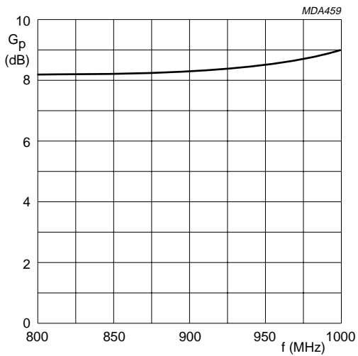
Fig.12 Power gain; class-AB operation; V_{CE} = 24\text{ V} ; P_L = 15\text{ W} ; R_{th\text{ mb-h}} = 0.4\text{ K/W} ; typical values.
