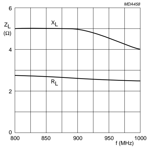
Fig.11 Load impedance; series components; V_{CE} = 24\text{ V} ; P_L = 15\text{ W} ; R_{th\text{ mb-h}} = 0.4\text{ K/W} ; typical values.
