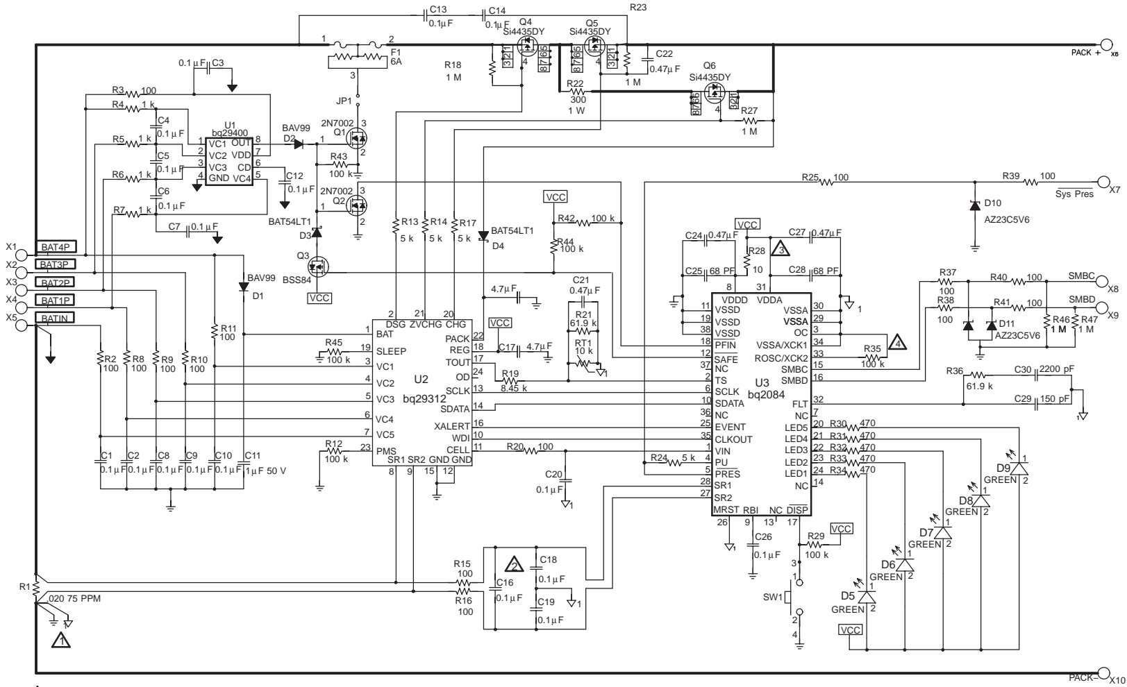
Figure 7. bq2084-V123 Based Battery Pack Schematic
