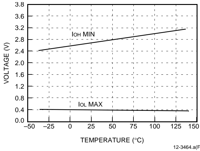
Figure 12. Minimum V_{OH} and Maximum V_{OL} vs. Temperature at V_{CC} = 4.5 V for the Receiver
