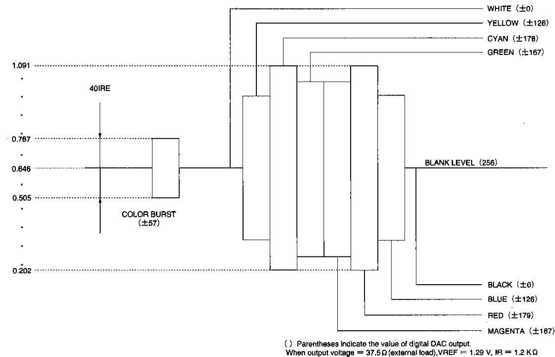
Fig. 2 NTSC C (chroma) signal output level
