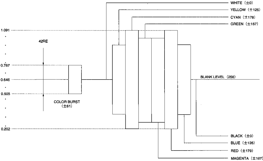
( ) Parentheses indicate the value of digital DAC output. When output voltage = 37.5 Ω (external load), VREF = 1.29 V, IR = 1.2 KΩ Fig. 5 PAL/PAL60 C (chroma) signal output level
