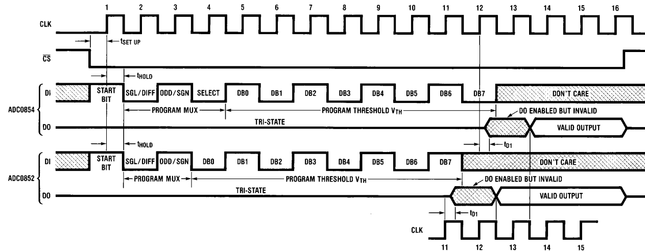
FIGURE 3. Timing Diagram
