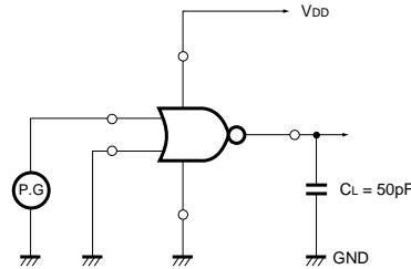
Fig.2 Switching characteristics
