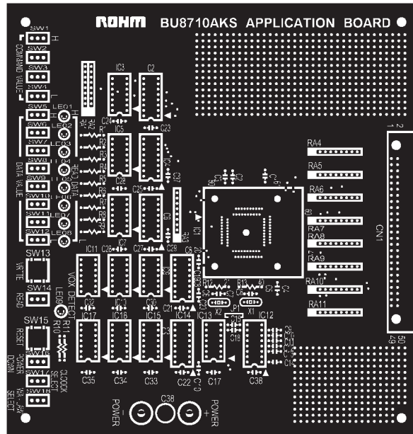
Fig. 27 Component layout
