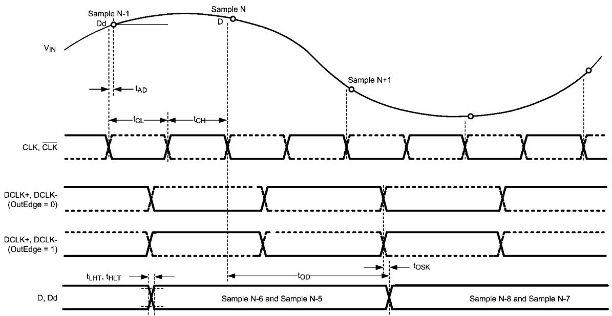
FIGURE 3. ADC081000 Timing
