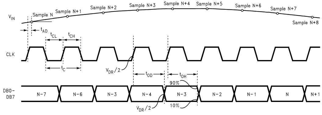
FIGURE 1. ADC08200 Timing Diagram
