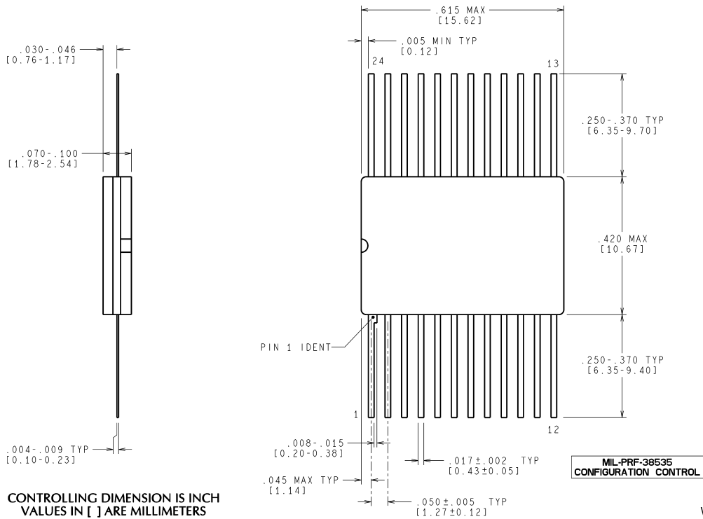
24-Lead Cerpack Package NS Package Number W24C
