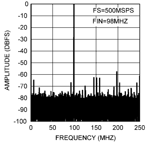
Spectral Response at f_{IN} = 98 MHz
