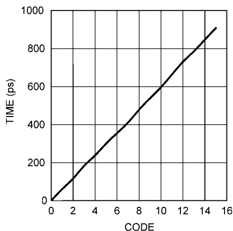
FIGURE 22. Typical Coarse Clock Phase Adjust Range
