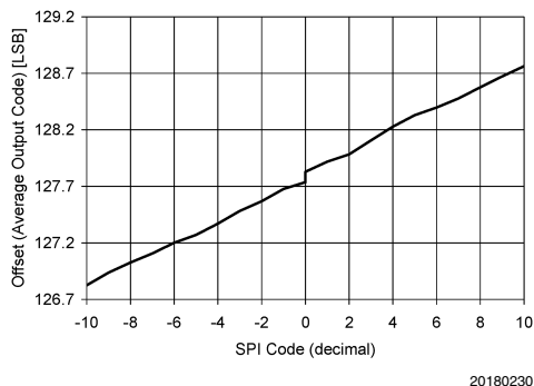
FIGURE 11. Extended Mode Offset Behaviour
