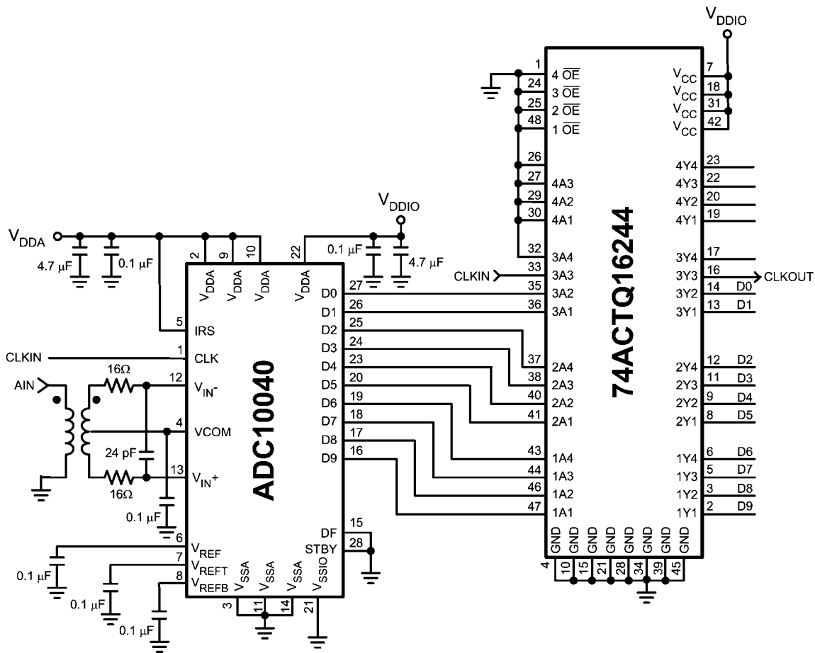
FIGURE 5. A Simple Application Using a Differential Signal Source
