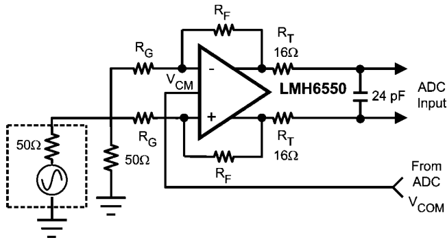
FIGURE 6. Using the LMH6550 for DC and wideband applications
