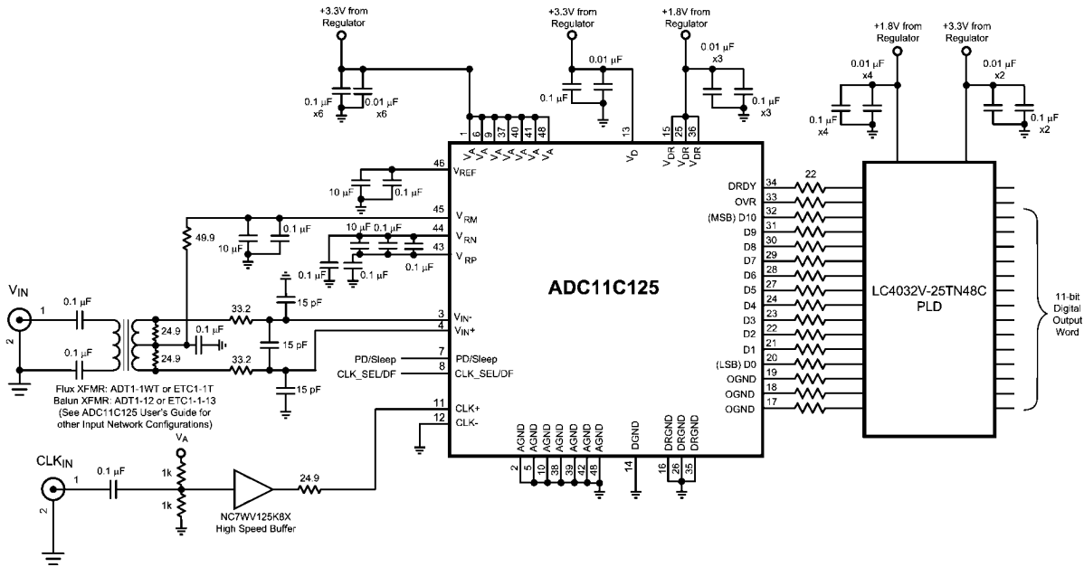
FIGURE 4. Application Circuit using Transformer Drive Circuit (If 14-bit compatibility is not required do not connect pins 17 - 19)
