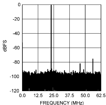
Spectral Response @ 398 MHz Input
