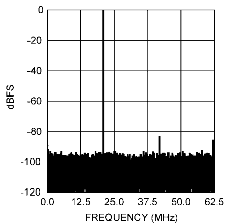
Spectral Response @ 146 MHz Input
