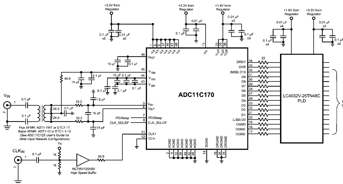
FIGURE 4. Application Circuit using Transformer Drive Circuit. If 14-bit compatibility is not required do not connect pins 17 - 19. If 12-bit compatibility is not required do not connect pin 19.
