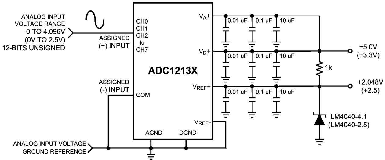
FIGURE 11. Single-Ended Biasing
