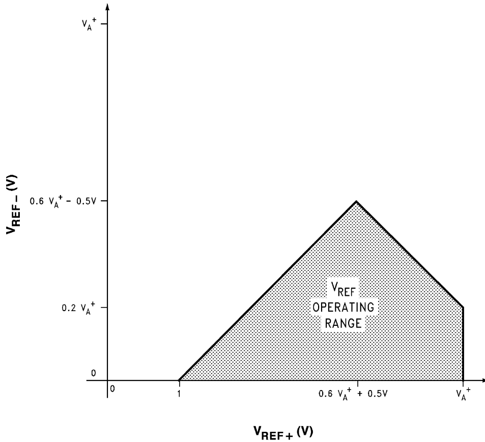
FIGURE 17. V_{REF} Operating Range
