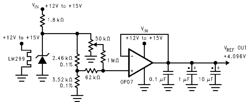
FIGURE 16. Low Drift Extremely Stable Reference Circuit
