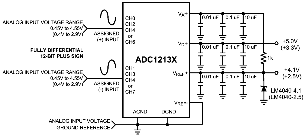
FIGURE 15. Fully Differential Biasing
